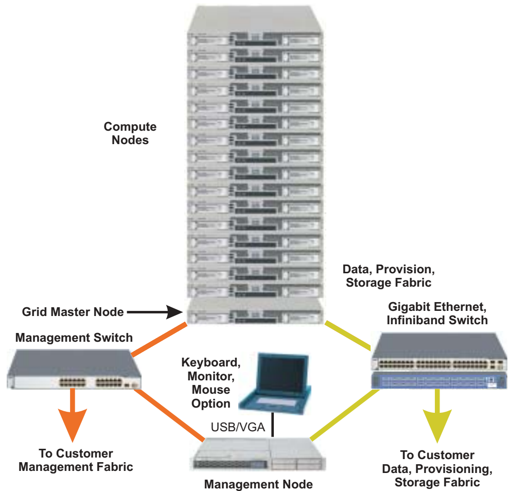
Figure 1. Sun Customer Ready HPC Cluster Architecture.
