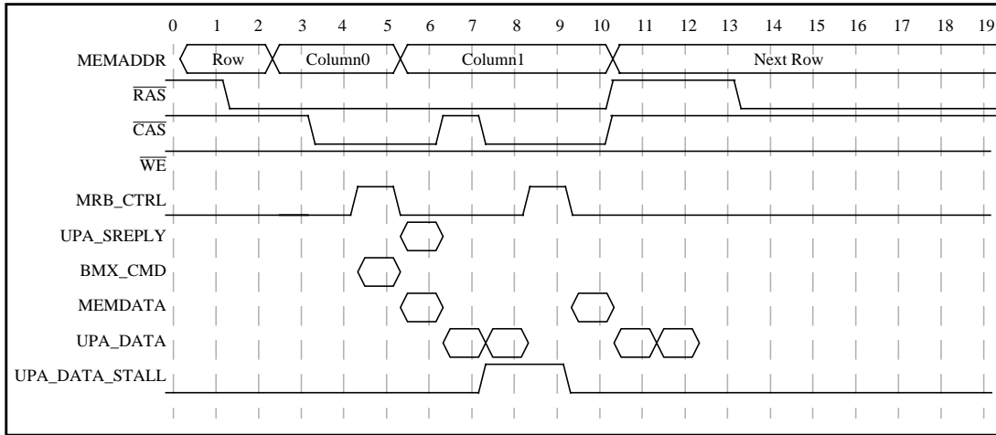
Figure 6-32 55.5-MHz CPU Read Timing
