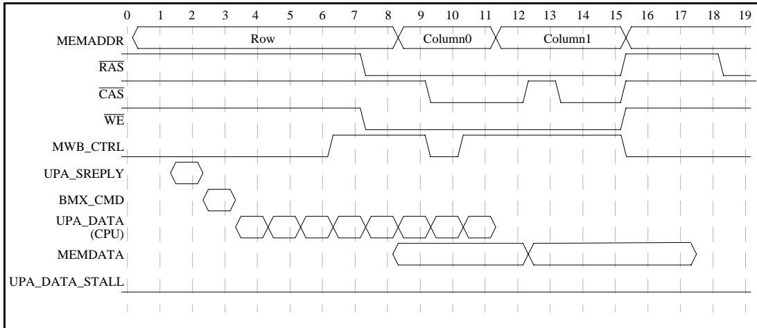
Figure 6-45 U2S Write Timing
