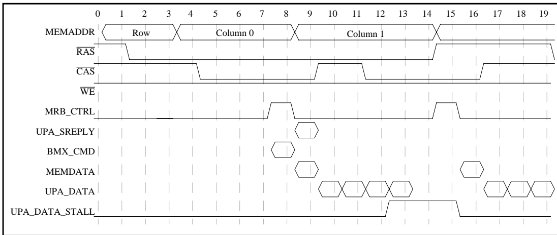
Figure 6-9 Default Memory U2S Read Timing
