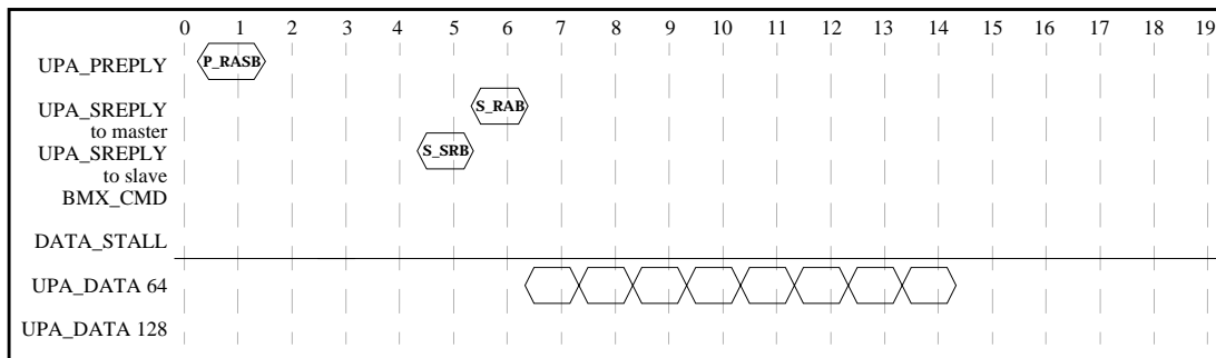
Figure 5-9 Best-Case Timing for Noncached Block Read, UPA64 -> UPA64
