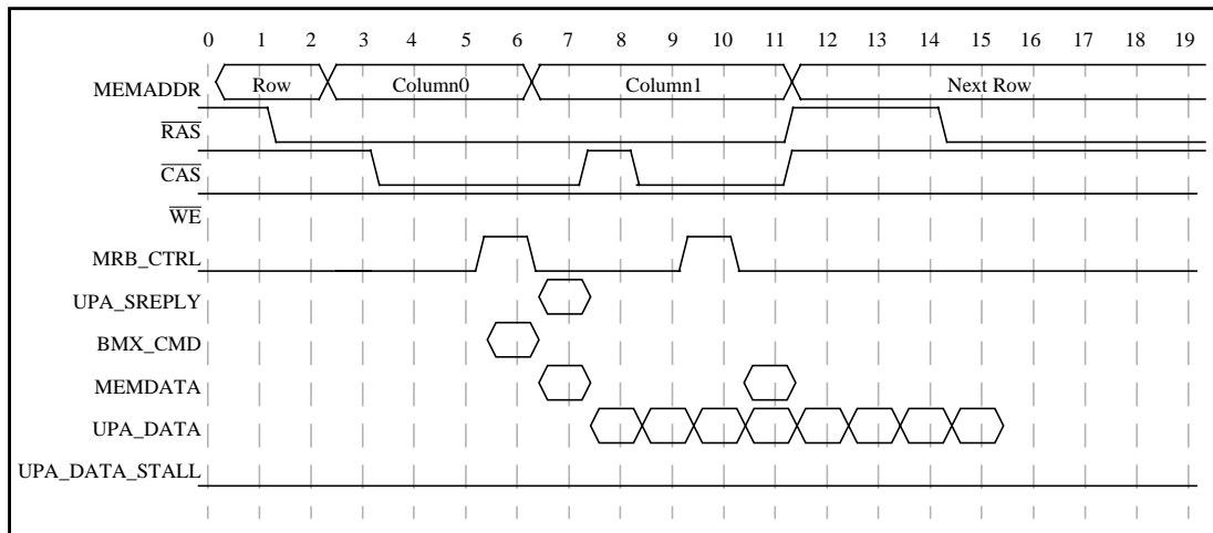
Figure 6-29 62.5-MHz U2S Read Timing
