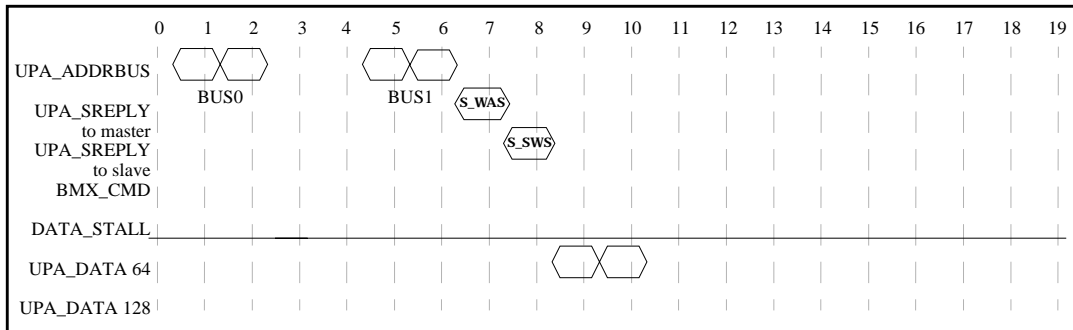
Figure 5-10 Best-Case Timing for Noncached Single Write, UPA64 -> UPA64
