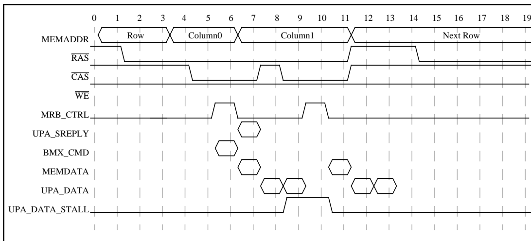
Figure 6-17 71.4-MHz CPU Read Timing
