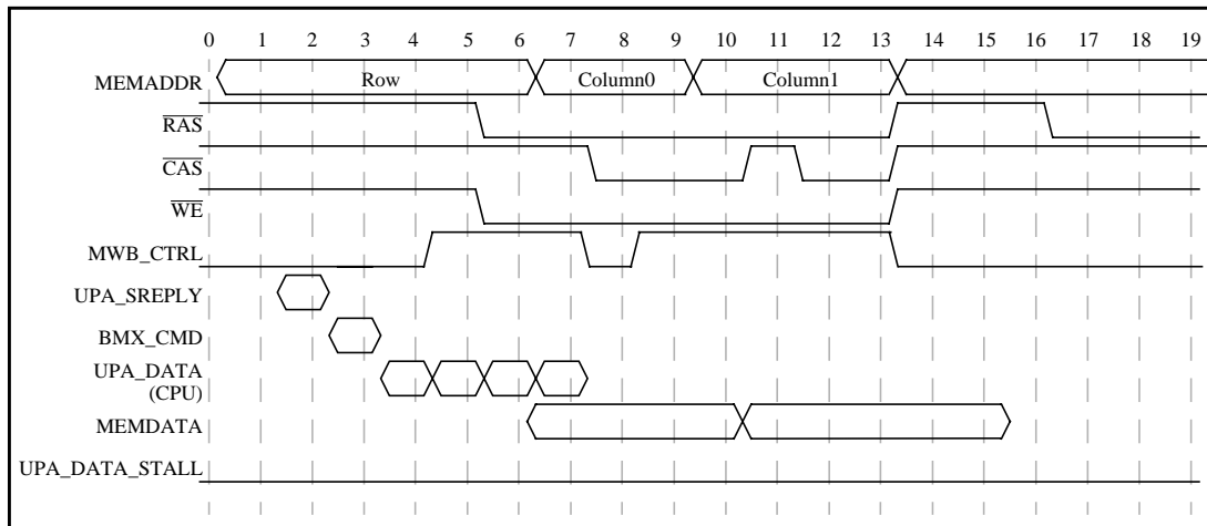
Figure 6-33 55.5-MHz CPU Write Timing
