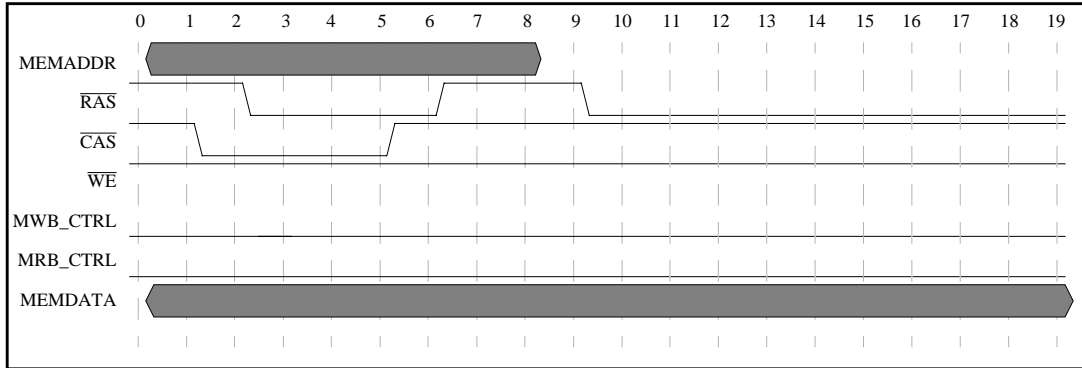
Figure 6-46 Refresh Timing
