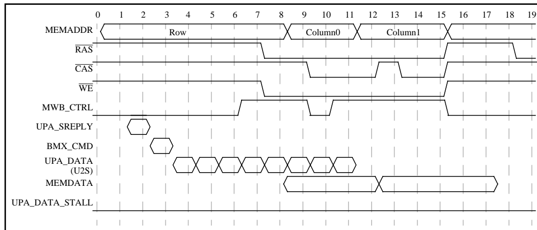
Figure 6-25 66.7-MHz U2S Write Timing
