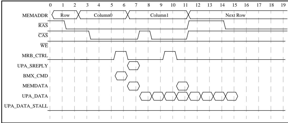
Figure 6-24 66.7-MHz U2S Read Timing
