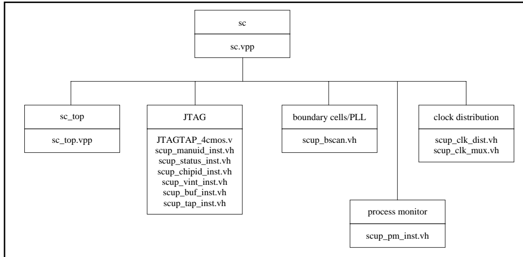
Figure 3-2 Top-Level Hierarchy
