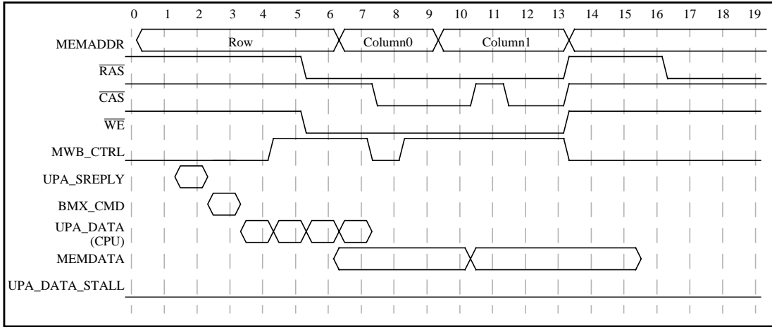
Figure 6-28 62.5-MHz CPU Write Timing
