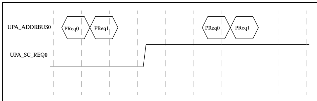
Figure 5-1 Best-Case PRequest-to-PRequest Timing (ABus0 to ABus0)
