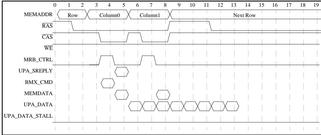
Figure 6-44 U2S Read Timing
