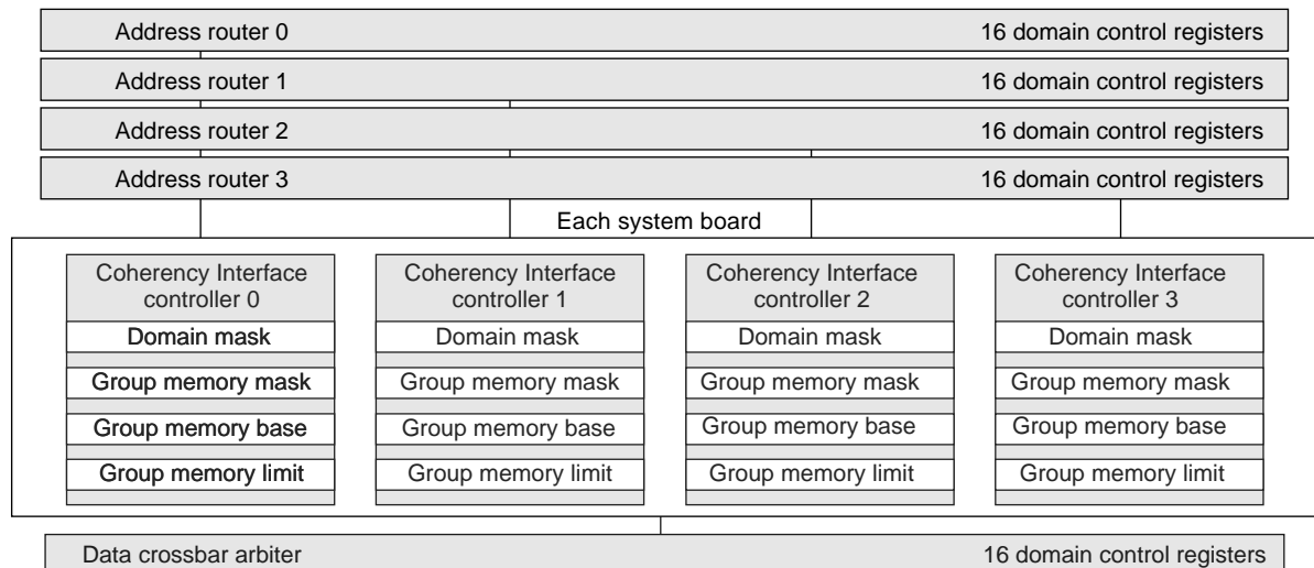
Figure 7. Domain registers in the Starfire interconnect.
