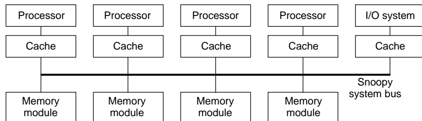
Figure 1. Symmetric multiprocessor.
