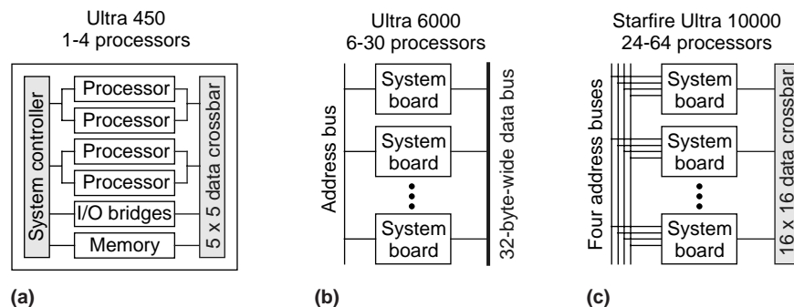
Figure 2. Three Ultra Port Architecture implementations: (a) a small system consisting of a single board with four processors, I/O interfaces, and memory; (b) a medium-sized system with one address bus and a wide data bus between boards; and (c) a large system with four address buses and a data crossbar between boards.
