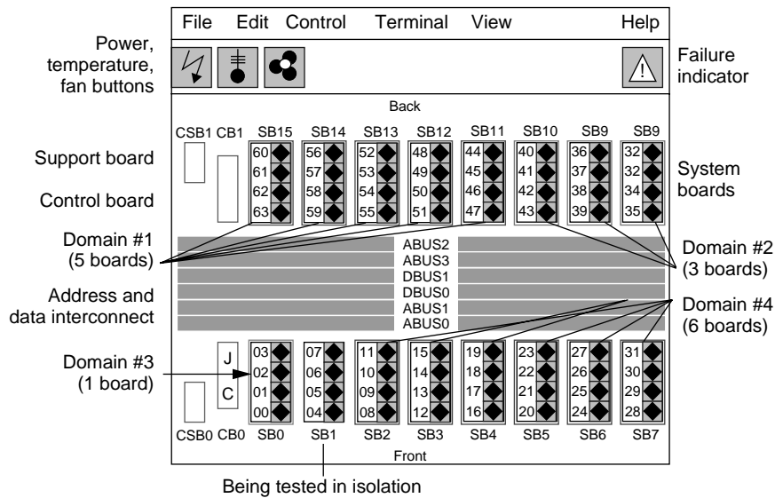
Figure 6. System service processor Hostview main screen.
