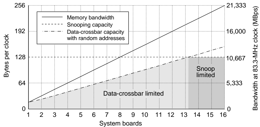
Figure 3. Snooping and data interconnect capacity.
