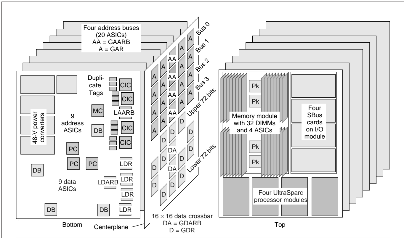
Figure 5. Bottom (left) and top (right) of the system boards, with the centerplane shown in the middle.
