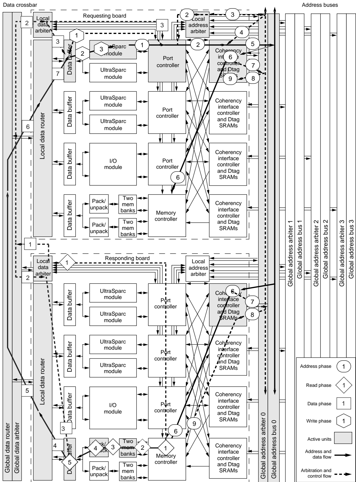
Figure 4. Interconnect steps for a load-miss from memory.
