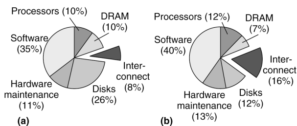
Figure 10. Interconnect cost percentages for (a) the Ultra 6000 with bus interconnect and (b) the Starfire Ultra 10000 with crossbar interconnect.
