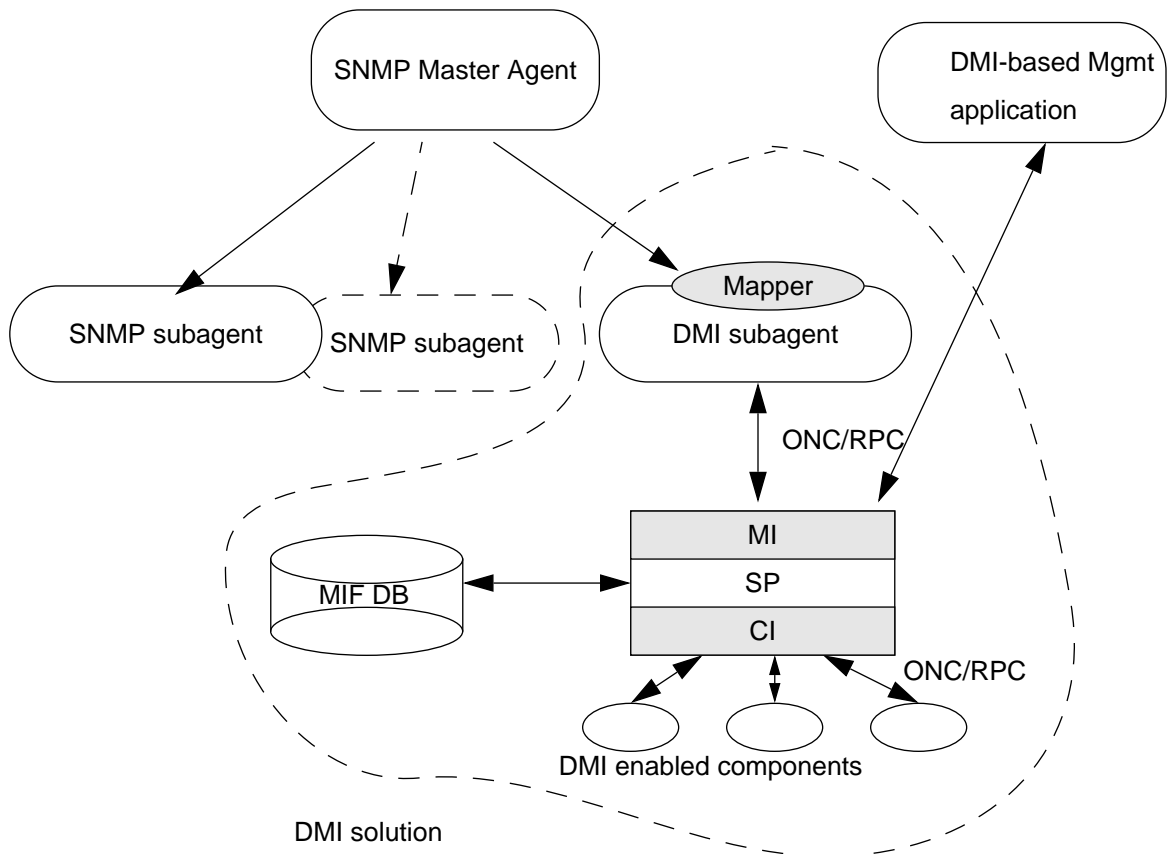
Figure 5-1 illustrates the overall architecture of how the DMI solution relates to the Enterprise Agents.
