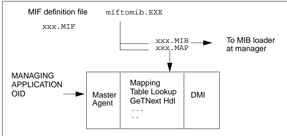
Figure 6-2 MIF-to-MIB Mapping
