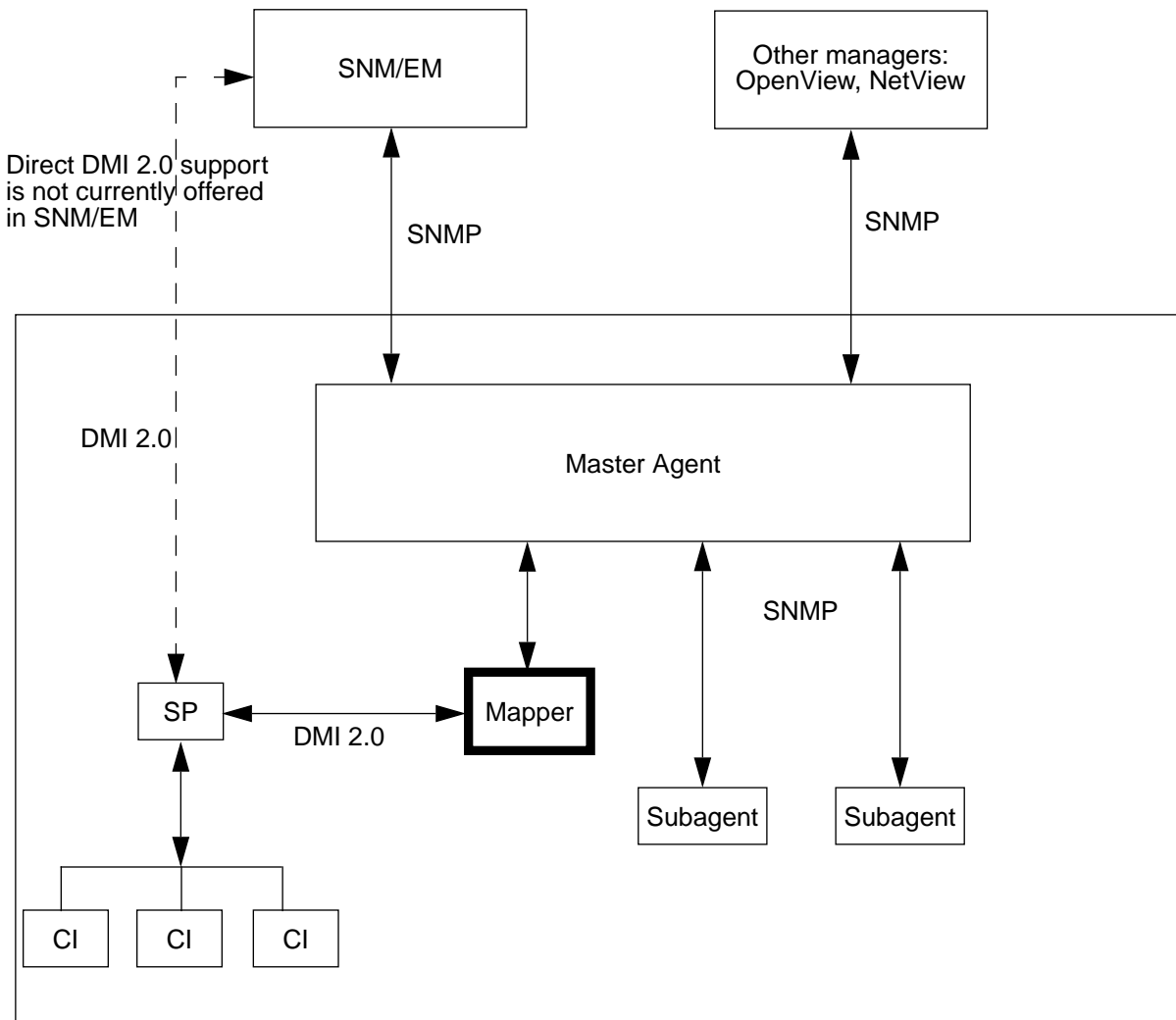
Figure 6-1 snmpXdmid Overview
