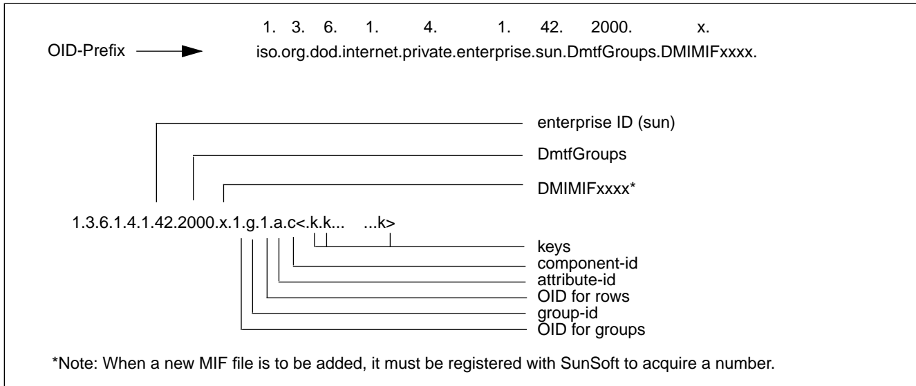
Figure 6-3 MIB OID Layout
