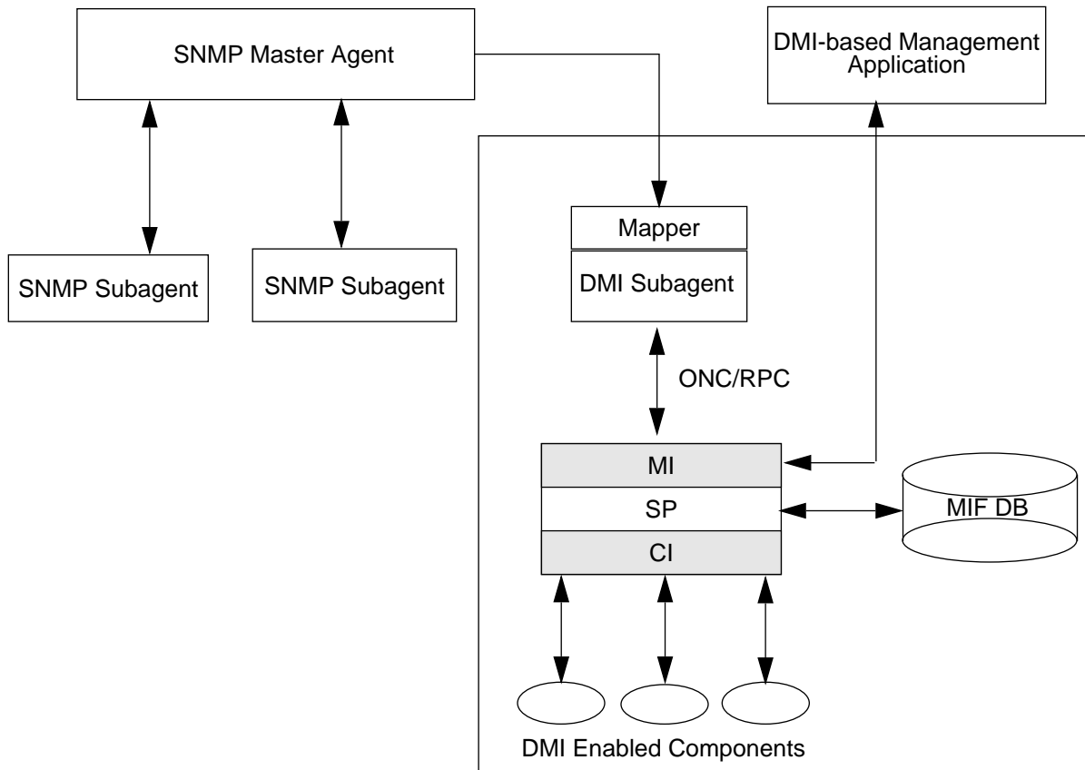
Figure 1-1 Architecture of the SEA
