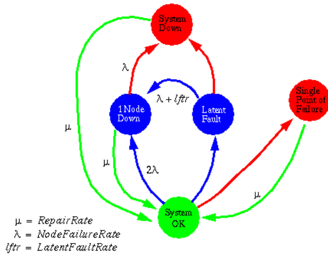
FIGURE 2 Markov Modeling
