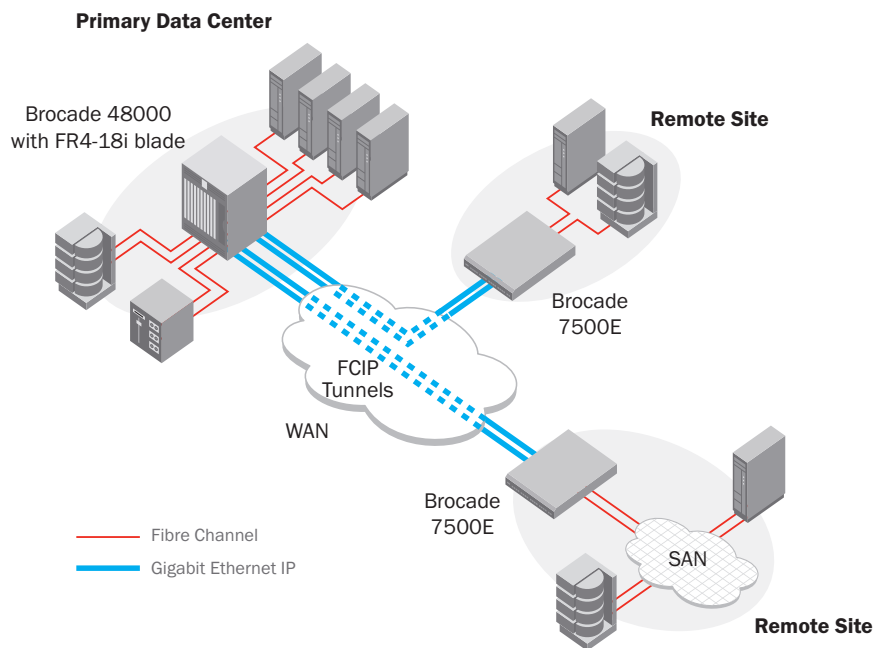
Figure 2. Interconnecting remote SAN fabrics to a central data center, the Brocade 7500E enables lower-cost remote data replication for centralized backup.
